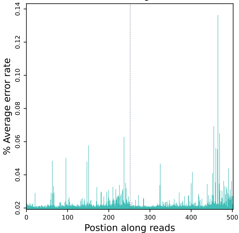
Error rate distribution along reads (R10707)
